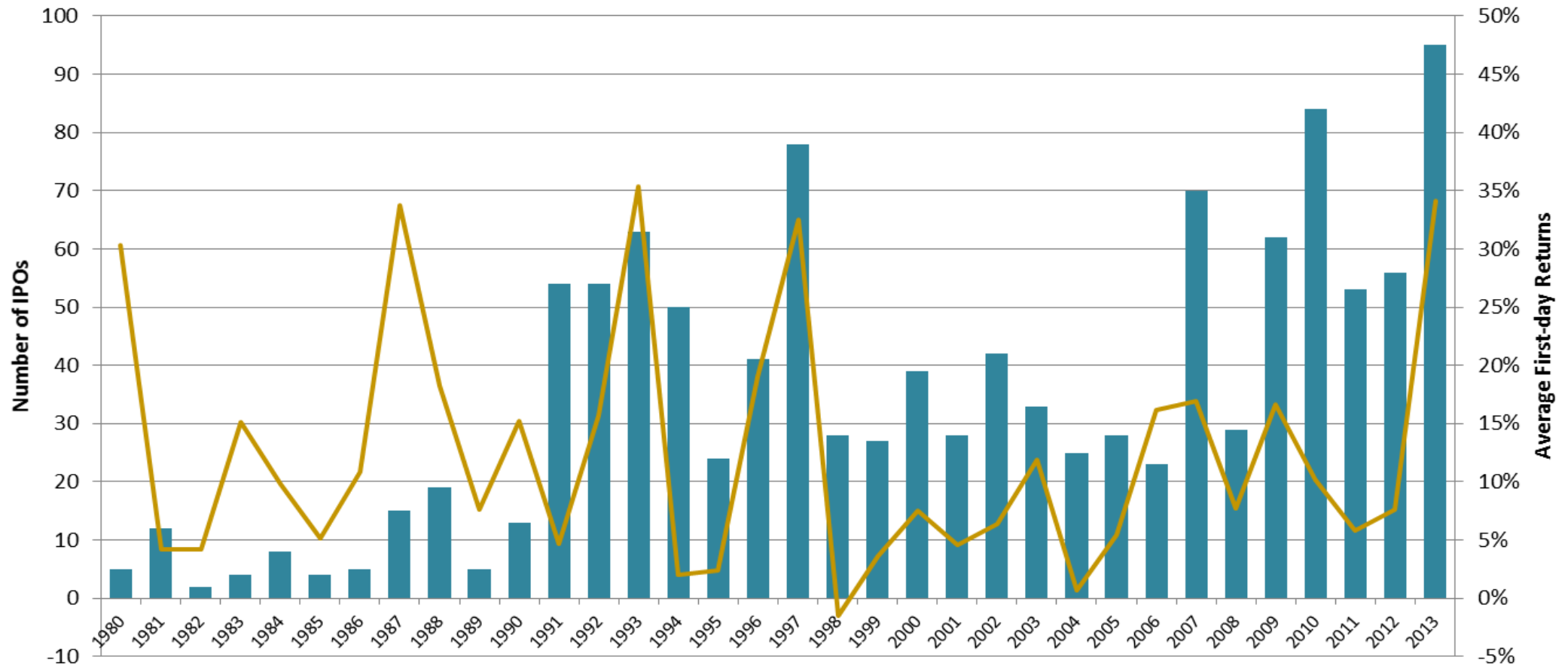
Number of Offerings (bars) and Average First-day Returns on Hong Kong IPOs, 1980 - 2013
