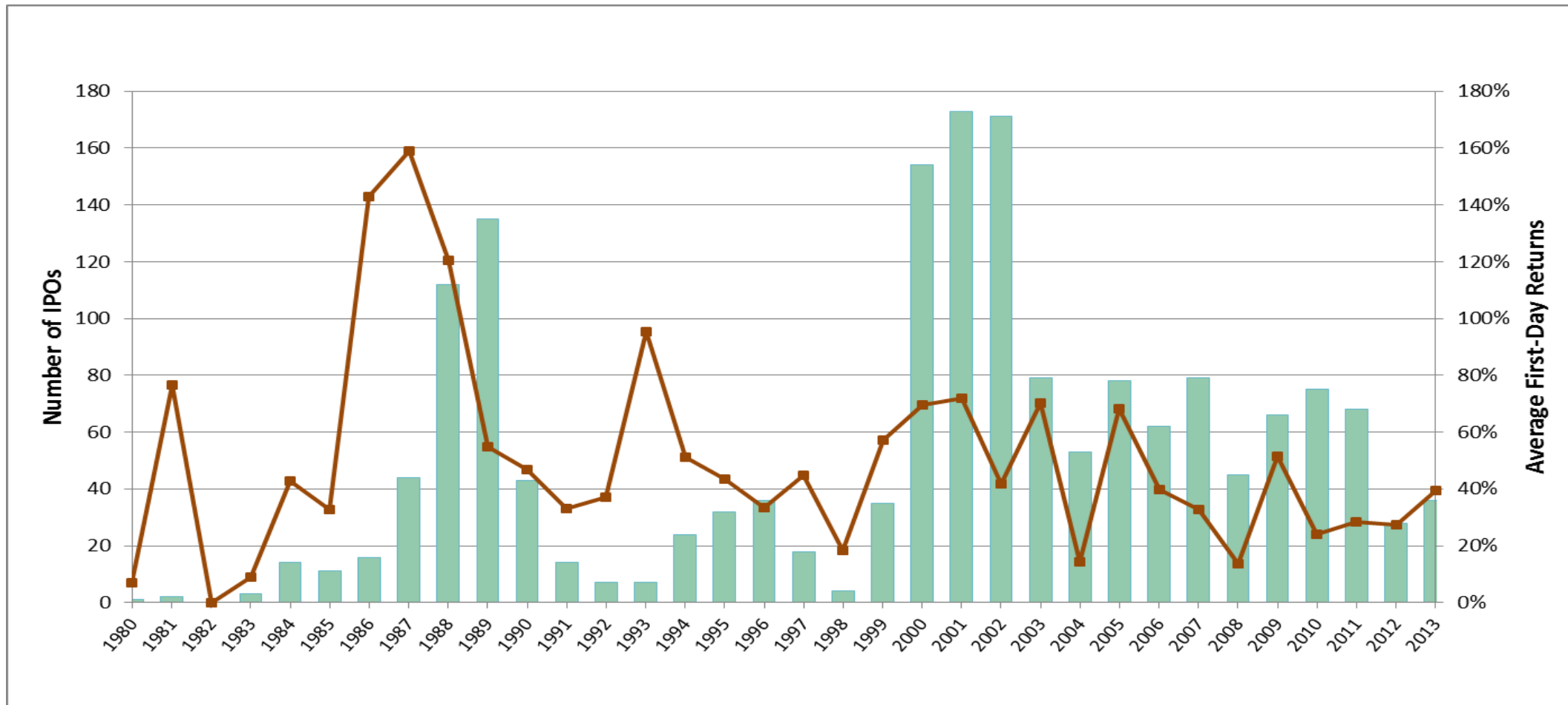
Number of Offerings and Average First-day Returns on Korean IPOs, 1980 - 2013
